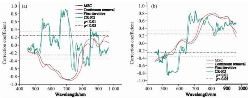
图 5 硬度与光谱变换数据的相关性(a), 弹性与光谱变换数据的相关性(b) Fig. 5 Correlation between hardness and spectral data transfer (a), correlation between springiness and spectral data transfer (b)
