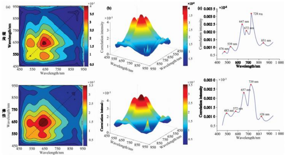
图 6 皮蛋凝胶质构特性二维相关同步谱(a), 三维立体图(b), 自相关谱(c) Fig. 6 (a) Two-dimensional correlation synchronization spectra of texture properties of preserved egg gel, (b) 3D stereo plots, (c) Autocorrelation spectra
