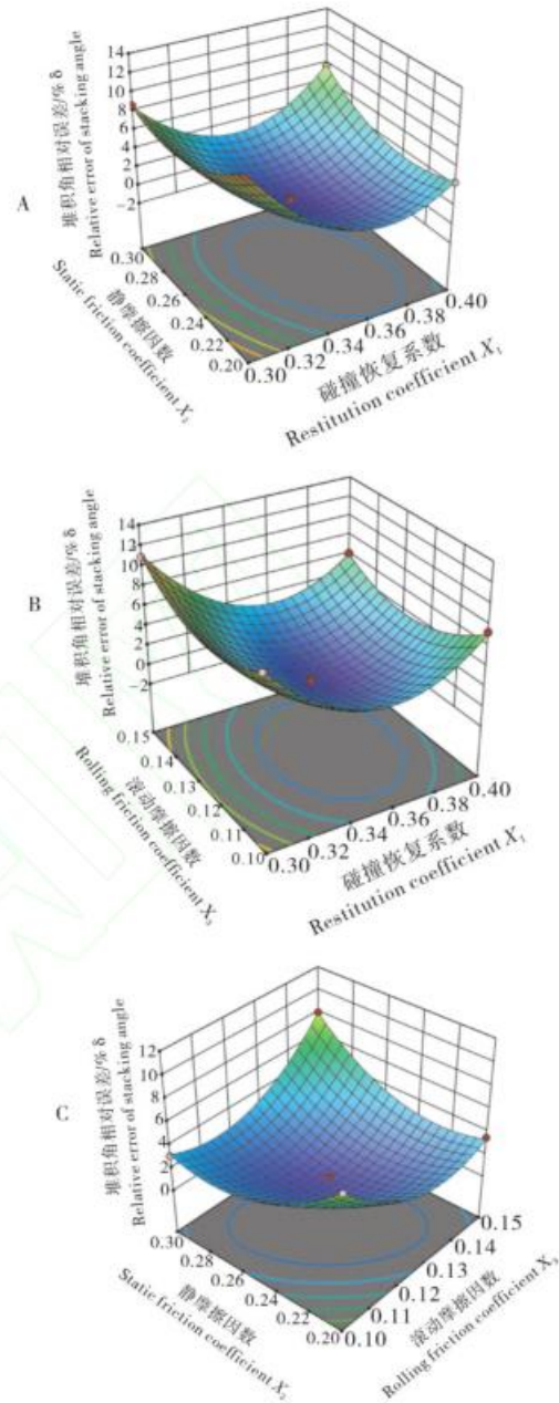
图8 试验因素对硬颗粒饲料堆积角相对误差的影响 Fig.8 Effects of experimental factors on relative error of Hard pellet feed stacking angle
